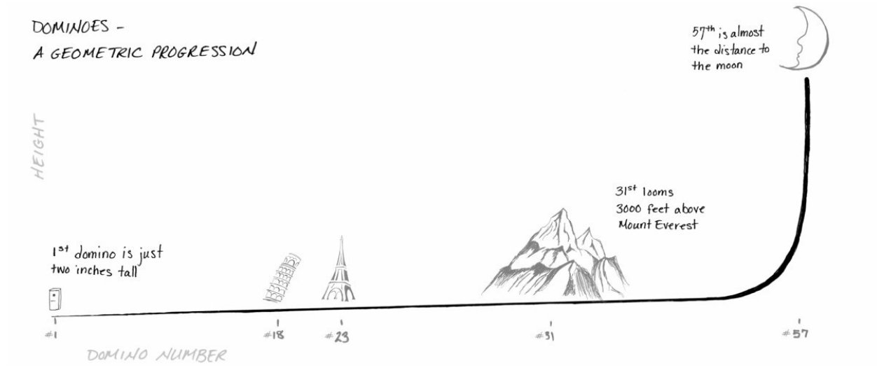
FIG. 2 A geometric progression is like a long, long train – it starts out too slow to notice until it’s moving too fast to stop.
